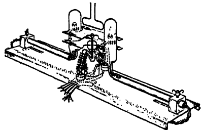
Parallel-plate ultrahigh-frequency-oscillator circuit for generating 10 to 15 watts of useful power at about 650 megacycles, and actual arrangement of tubes and parts.
